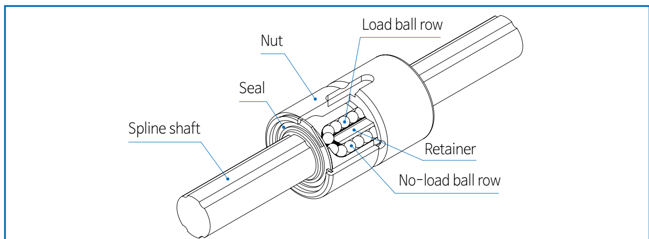
Figure 12. Structure of linear ball spline
