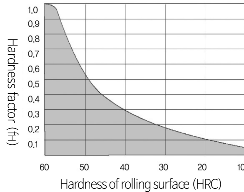
Figure 2. Hardness factor( f_H )
