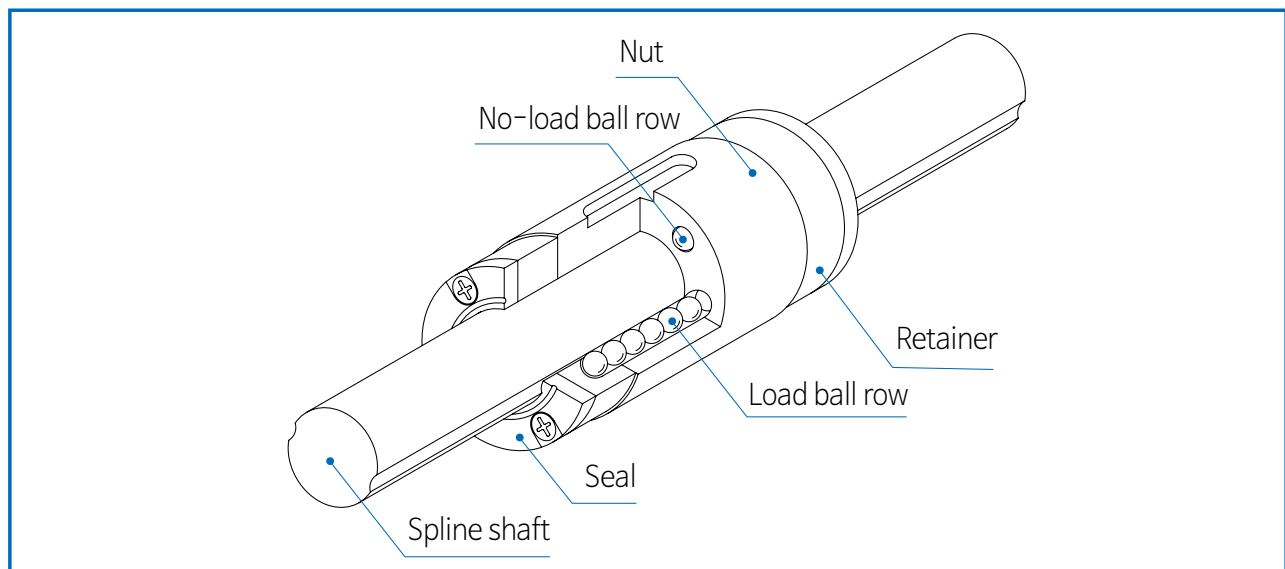
Figure 11. Structure of compact ball spline
